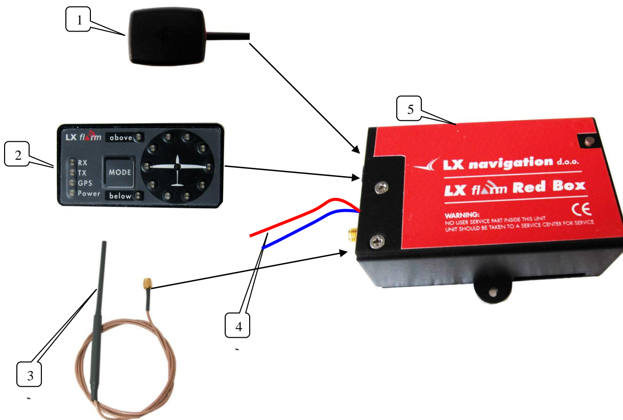
1 GPS antenna, 2 Flarm display, 3 RF antenna, 4 power lines, 5 Flarm box
